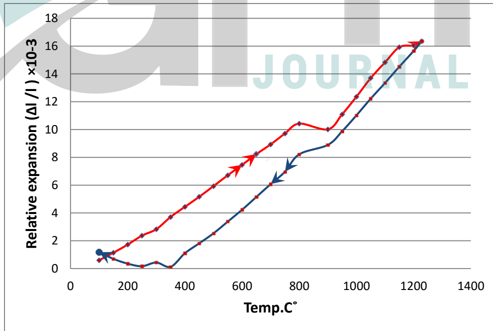
Fig.-1- Dilatation during heating and cooling at rate of 10 C°/min of HSS –R18
