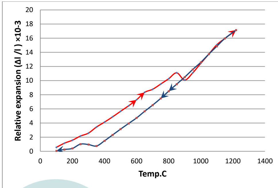
Fig.-2- Dilatation during heating and cooling at rate of 20C°/min of HSS –R18
