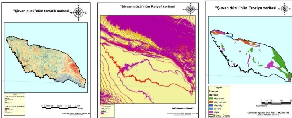
Figure4: Thematic map of the length/slope(LS)factor Figure 6: Soil erosion classification map.
