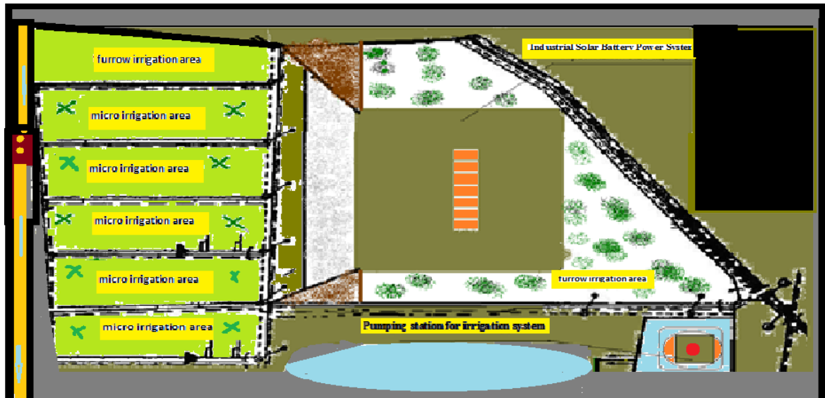
Fig.2. Scheme of the irrigation sprinkling station on the experimental part of the Terter RACS in the Garabagh land in the period 2006-2010 with the use of the Idad and MDR sprinklers:
